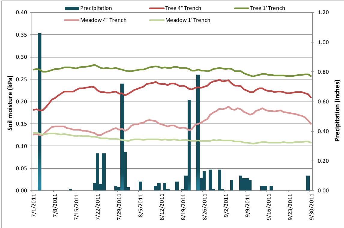
Figure 5. Comparison of Tree and Meadow soil moisture levels at the 4-inch and 1-foot depths, along with precipitation, July–September 2011.
