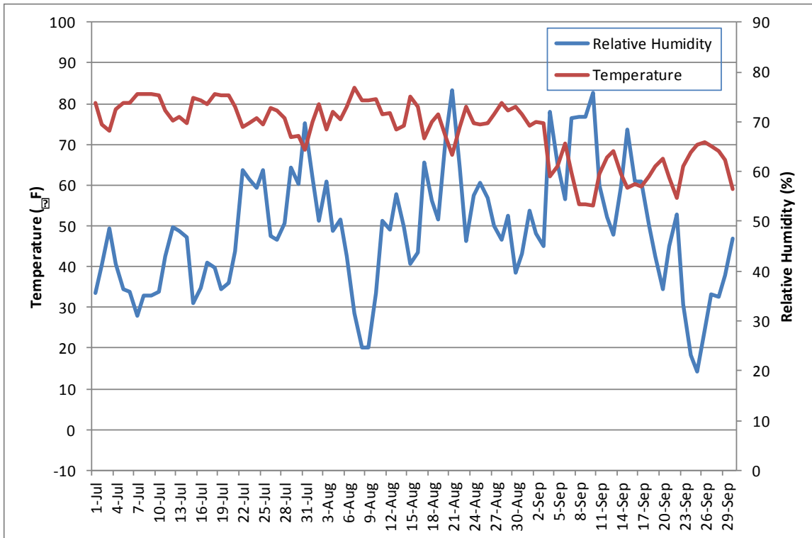
Figure 8. Daily average ambient air temperature and relative humidity, July–September 2011.
