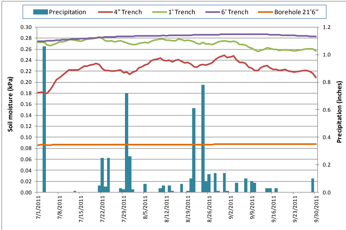
Figure 2. Tree site soil moisture levels (kPa) at four depths and daily precipitation amount (inches), July–September 2011.
