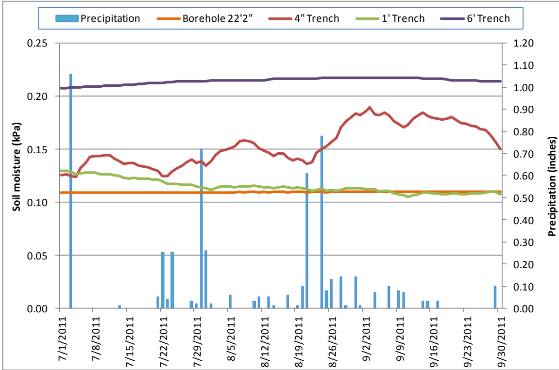
Figure 3. Meadow site soil moisture levels (kPa) at four depths and daily precipitation amount (inches), July–September 2011.
