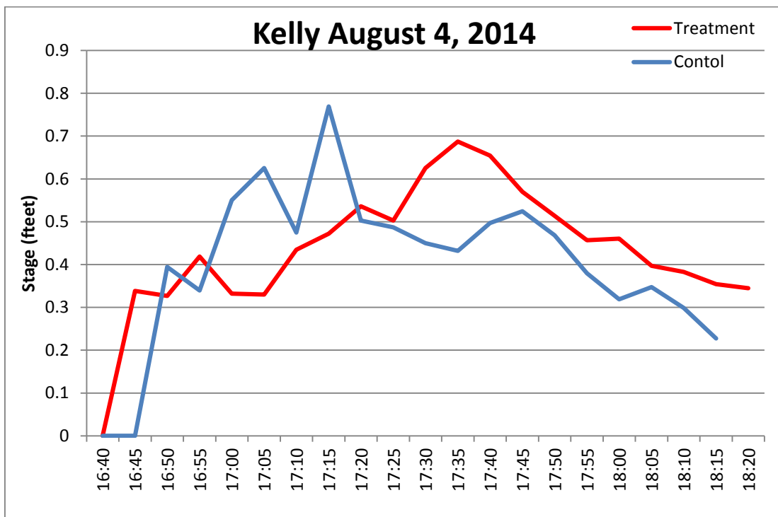
Figure 2.39. Hydrograph showing the Kelly treatment and control treatment during a storm flow event on August 4, 2014.
