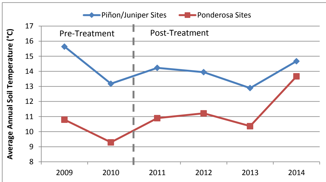
Figure 2.16. Annual average soil temperature values at the piñon/juniper and ponderosa pine sites, 2009–2014.
