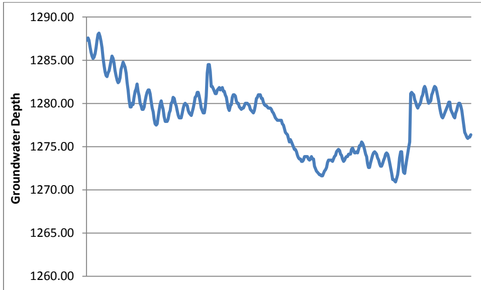
Figure 3.3. Well data from the Chilili site showing a declining water level until the snowmelt, which generates a small rise in groundwater depth.
