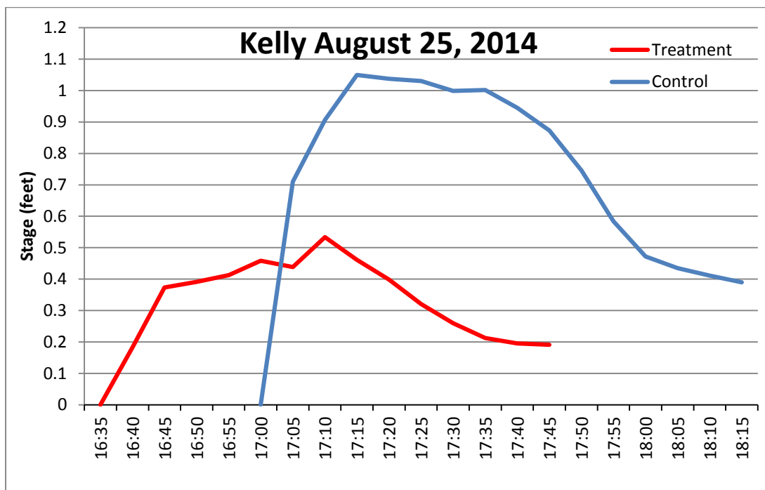
Figure 2.40. Hydrograph showing the storm flow at the Kelly treatment and control site that occurred on August 25, 2014.
