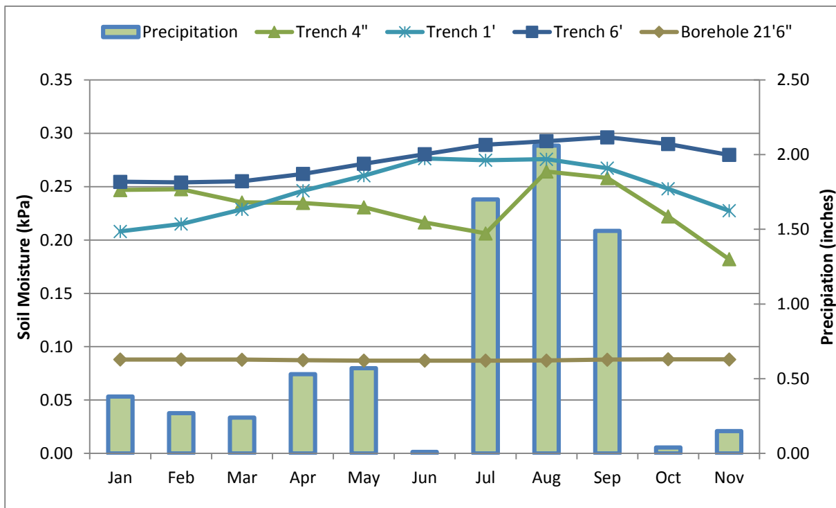
Figure 4.3. Tree site monthly average soil moisture and total precipitation for 2014.
