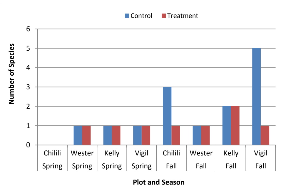
Figure 2.63. Numbers of rodent species recorded from thinning treatment and control plots across the four study sites in both spring and fall, 2014.
