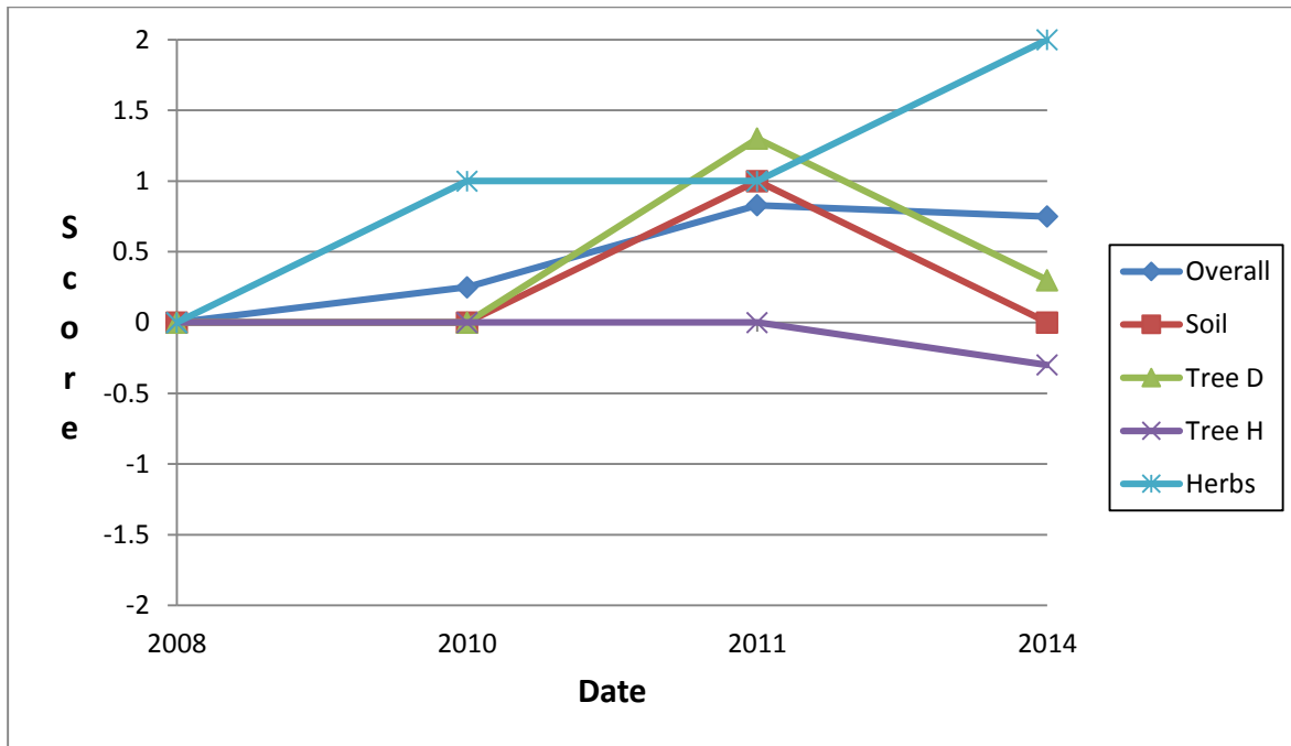
Figure 2.55. Parameter trend scores based on repeat photo point interpretation for the Vigil piñon/juniper treatment plot from 2008 through 2014.
