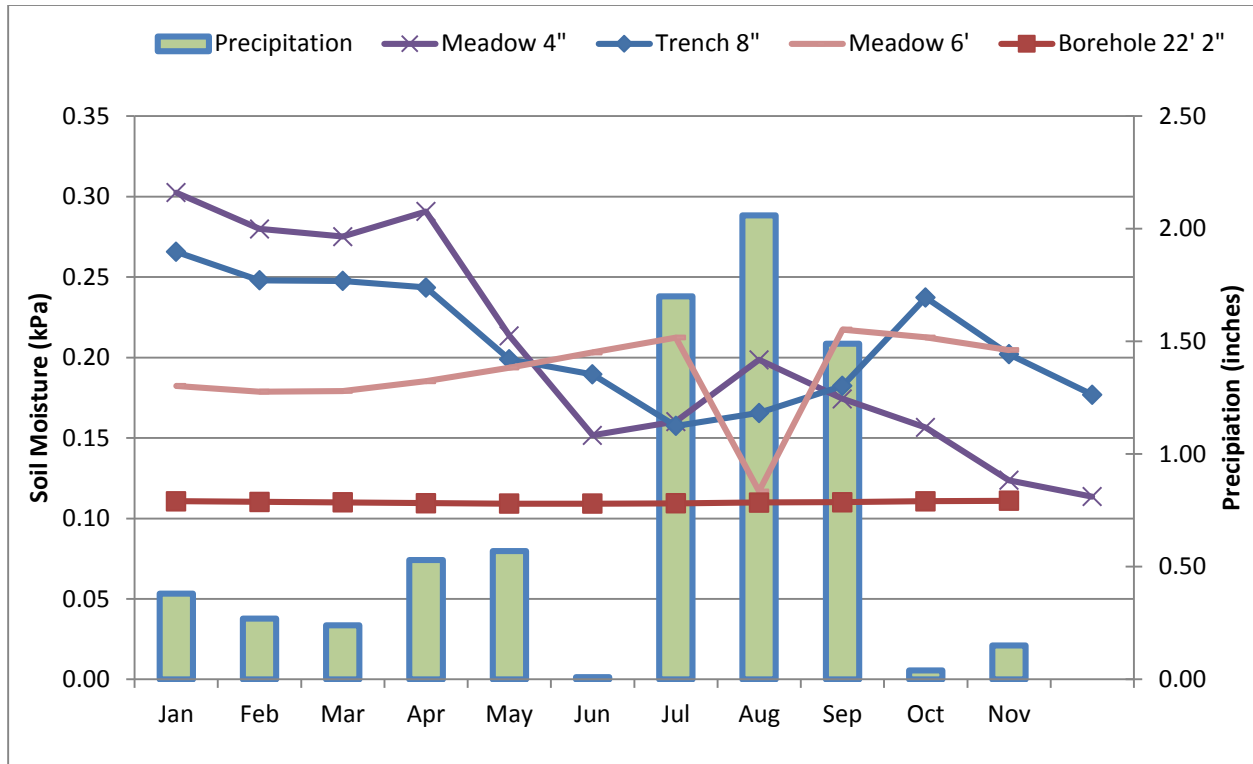
Figure 4.4. Meadow site average monthly soil moisture and total precipitation for 2014.
