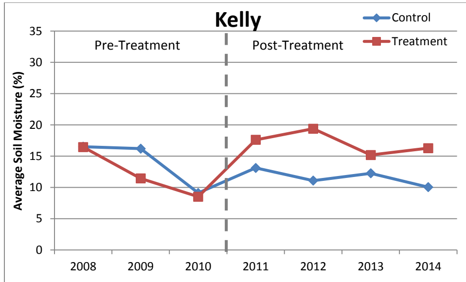
Figure 2.20. Average annual soil moisture readings taken at the Kelly site, 2008–2014.
