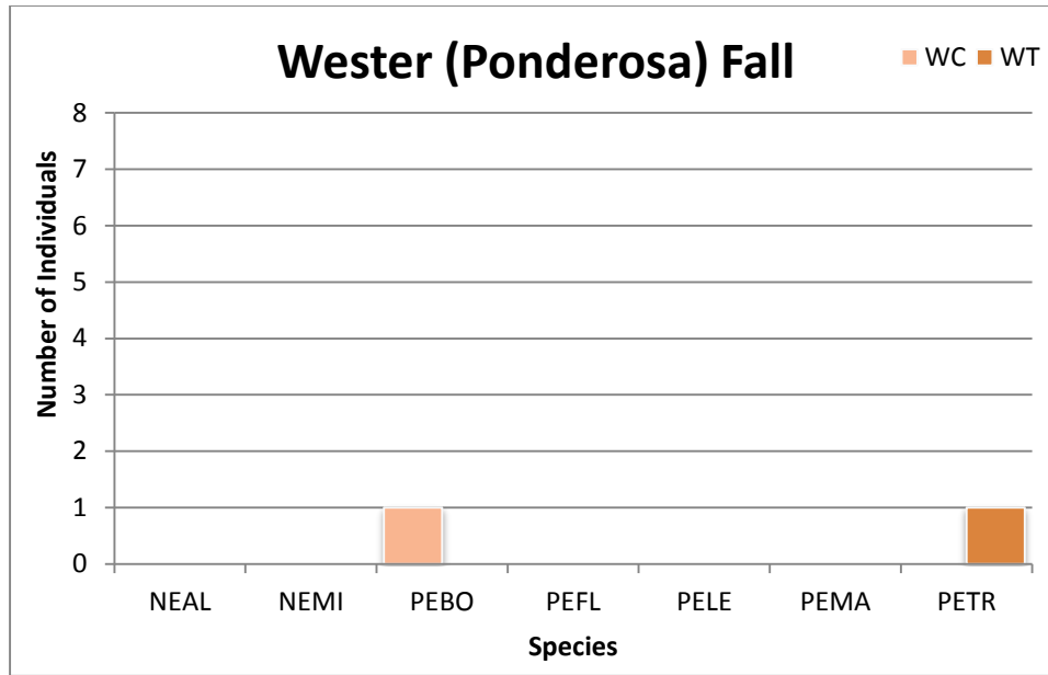
h. Wester control and treatment plots, fall 2014.
