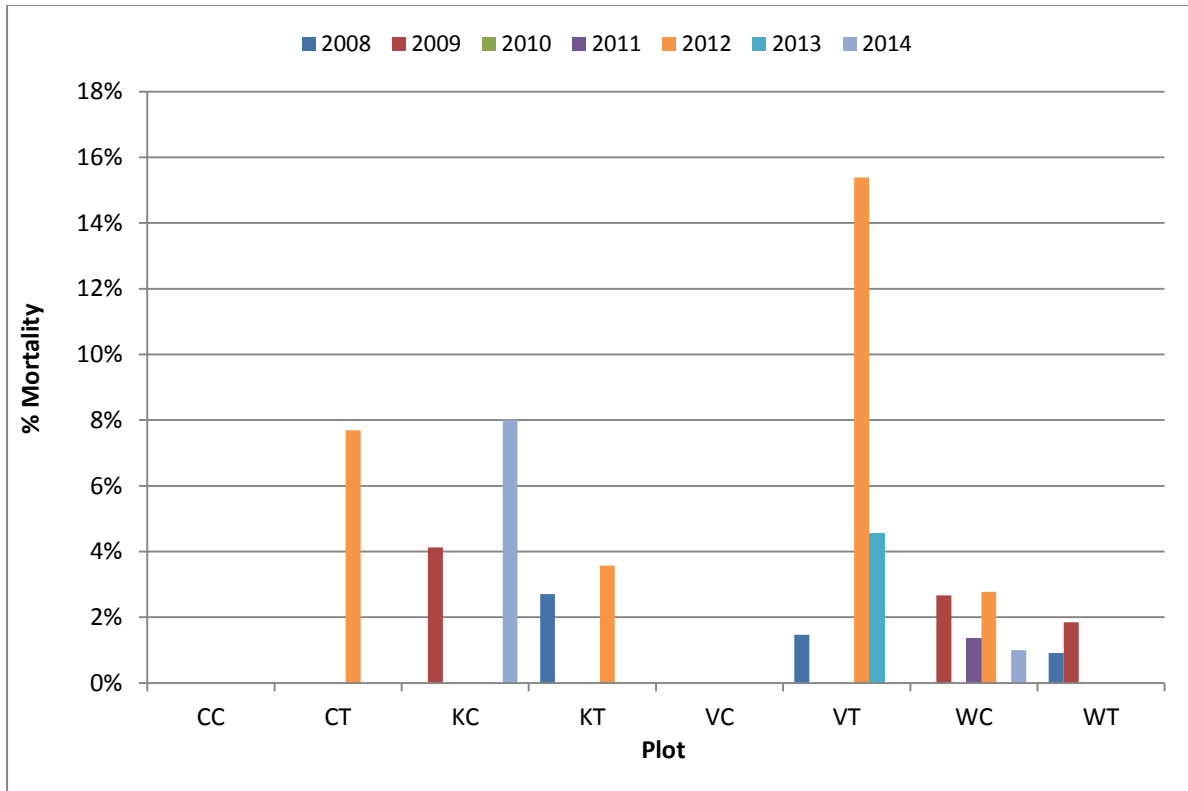
Figure 2.47. Percent tree mortality recorded across all thinning plots from 2008–2014. Percent mortality is recorded in relation to tree status in 2008.
