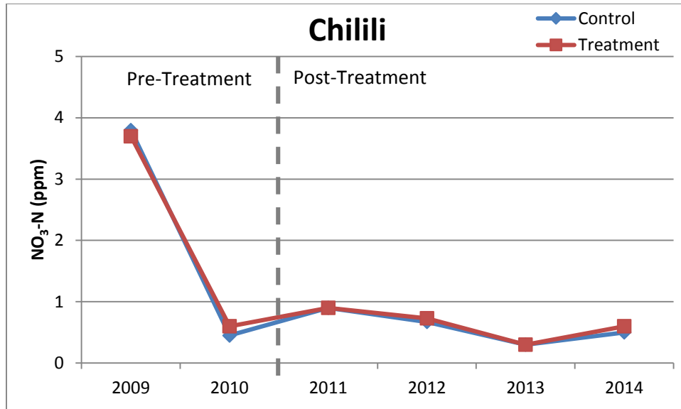
Figure 2.34. Nitrate concentrations measured at the Chilili sites, 2009–2014.
