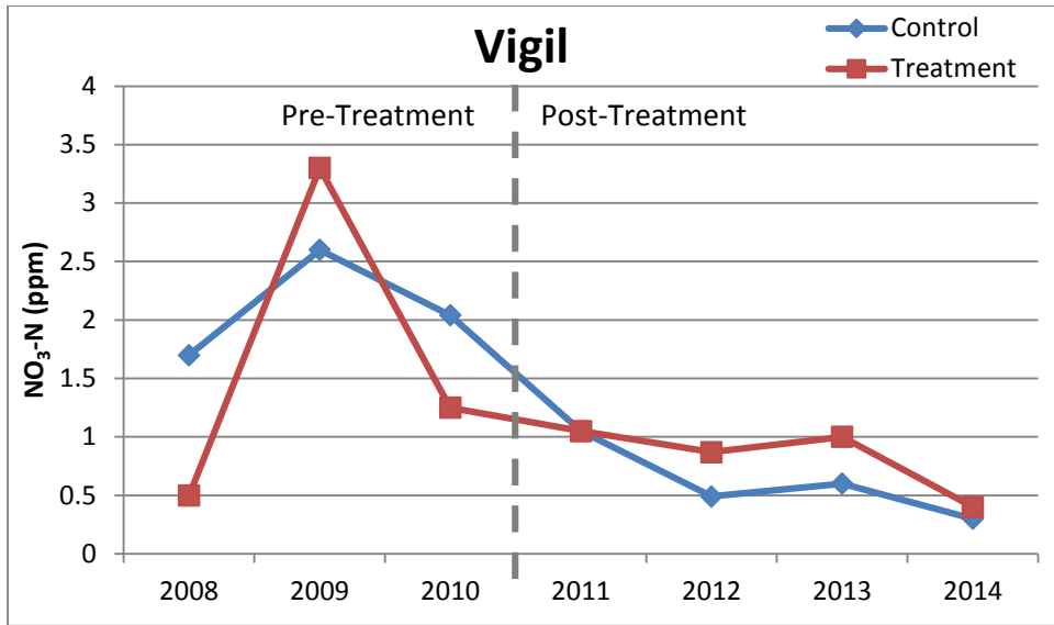
Figure 2.36. Nitrate concentrations measured at the Vigil sites, 2008–2014.
