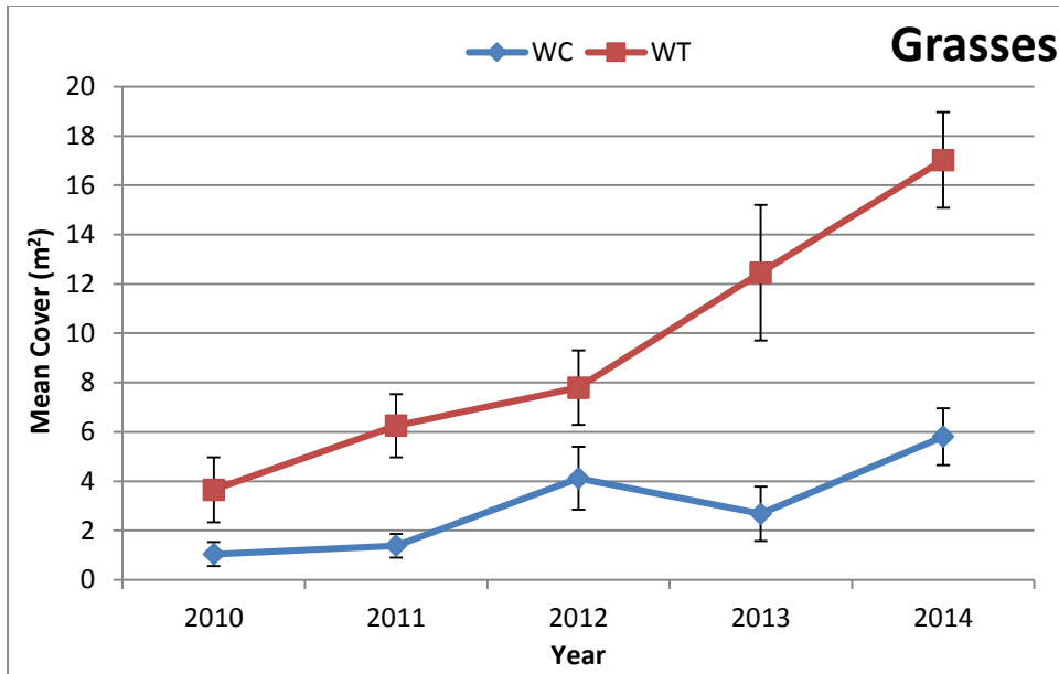
l. Grass, Wester.
