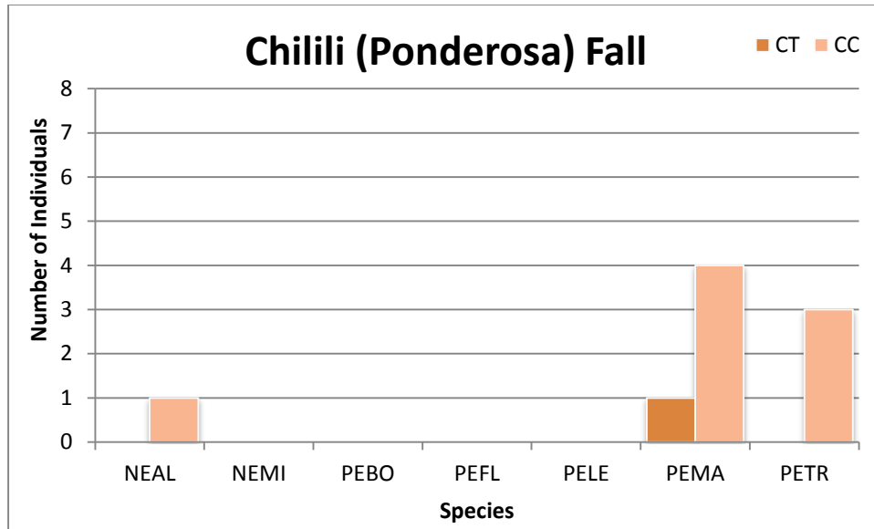
b. Chilili control and treatment plots, fall 2014.
