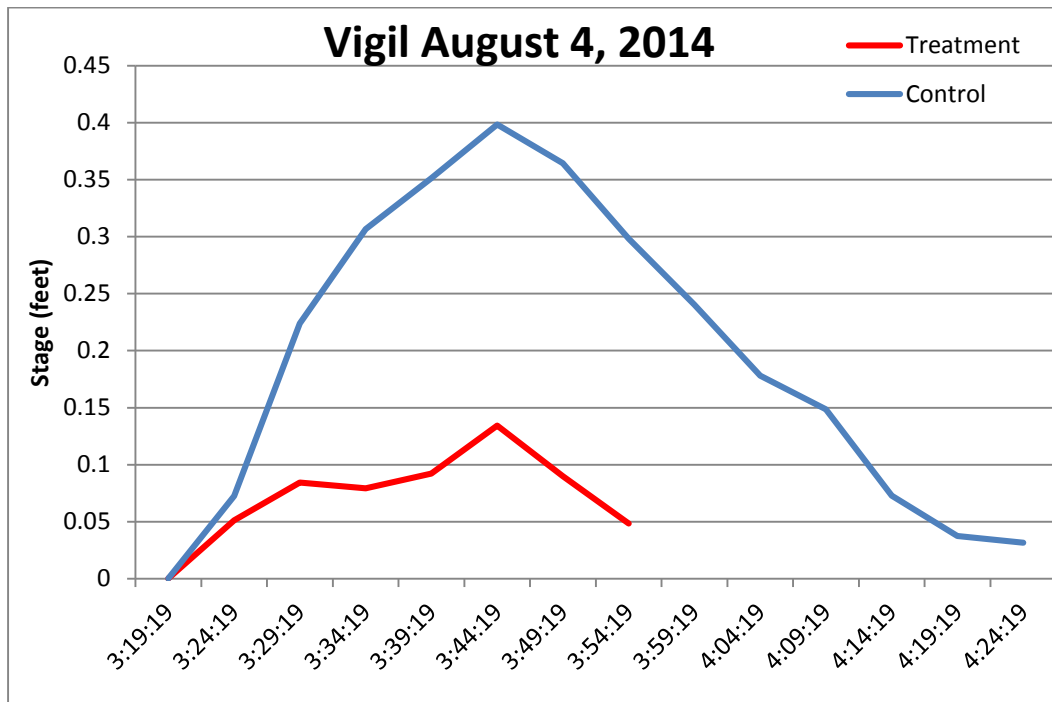
Figure 2.41. Hydrograph showing the storm flow at the Vigil treatment and control r site that occurred on August 4, 2014.
