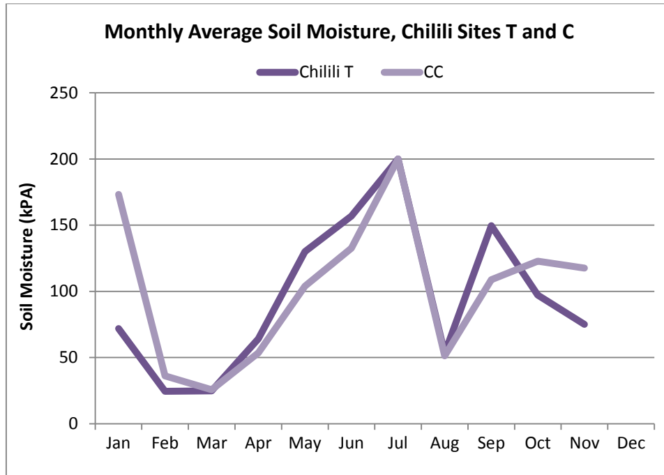
Figure 2.14. Monthly average soil moisture tensions (–10 cm) from the two paired Chilili ponderosa pine study plots in 2014.
