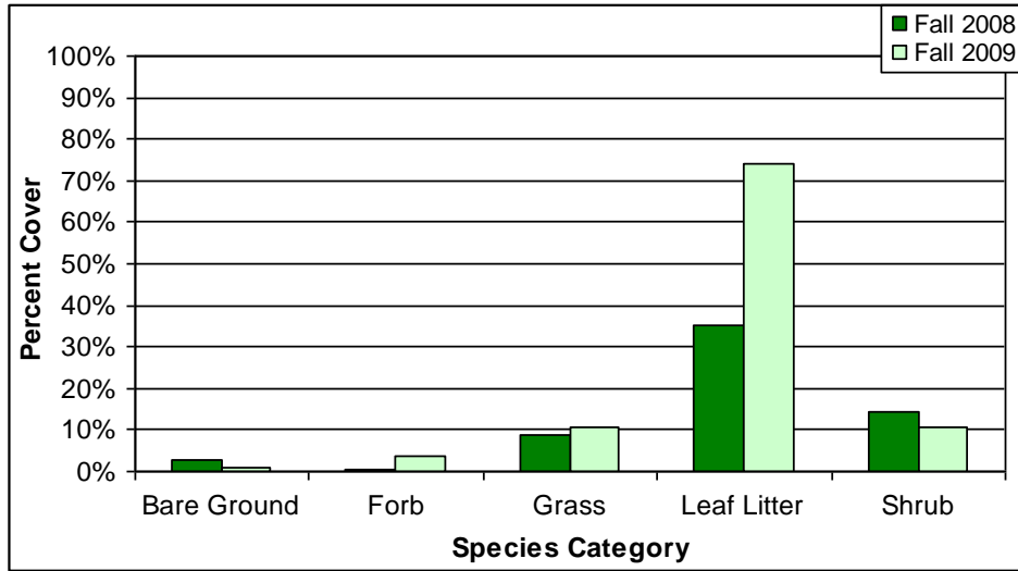
Figure 3.12. Percentage of cover by growth form for Bouton unburned plot 7, fall 2008–2009.
