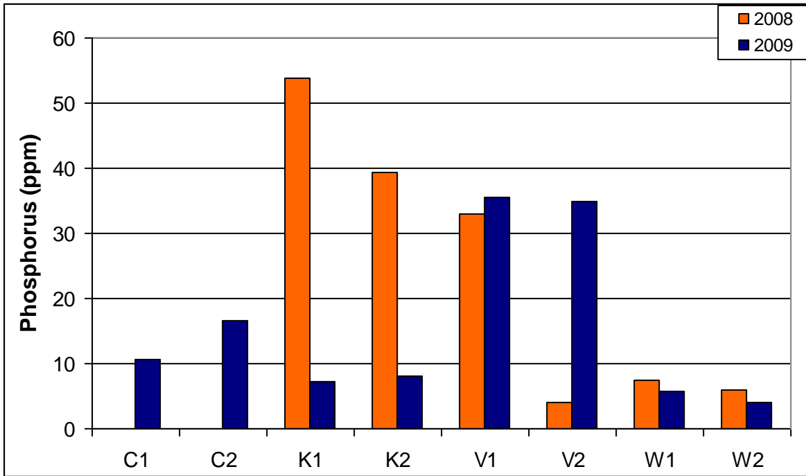
Figure 2.26. Baseline concentrations of phosphorus measured on all the thinning plots during 2008 and 2009; C= Chilili, K = Kelly, V = Vigil, and W = Wester.
