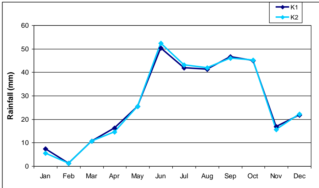
Figure 2.3. Monthly cumulative precipitation (rainfall and snow) from the two paired Kelly piñon/juniper study plots.
