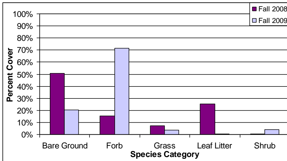
Figure 3.11. Percentage of cover by growth form for Bouton high-severity plot 2, fall 2008–2009.
