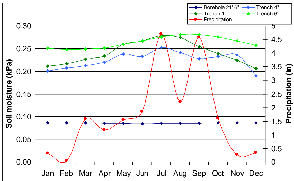
Figure 5.3. Tree site monthly average soil moisture and total precipitation for 2009.
