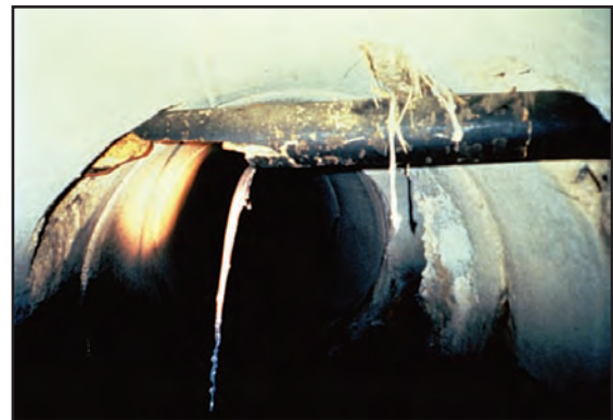
Figure 1: Sewer Pipe Discharging to the Storm Drain System
