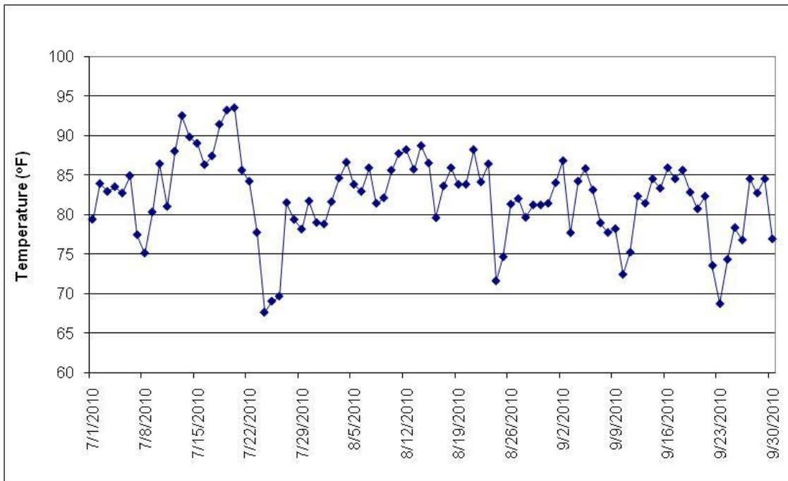
Figure 7. Daily maximum ambient air temperature (fahrenheit) recorded daily, July 1-September 30, 2010
