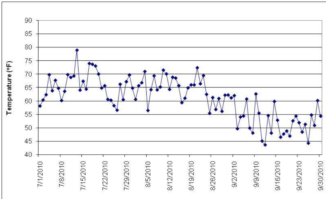
Figure 6. Daily minimum ambient air temperature (fahrenheit) recorded daily, July 1-September 30, 2010.
