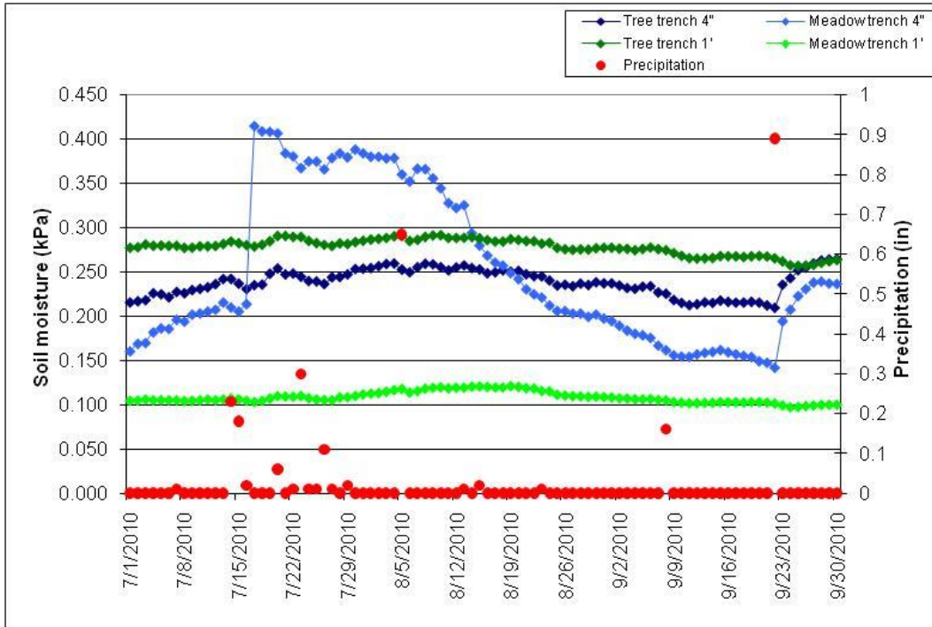
Figure 5. Comparison of Tree and Meadow soil moisture levels at the 4\", and 1' depths, along with precipitation, July 1-September 30, 2010.
