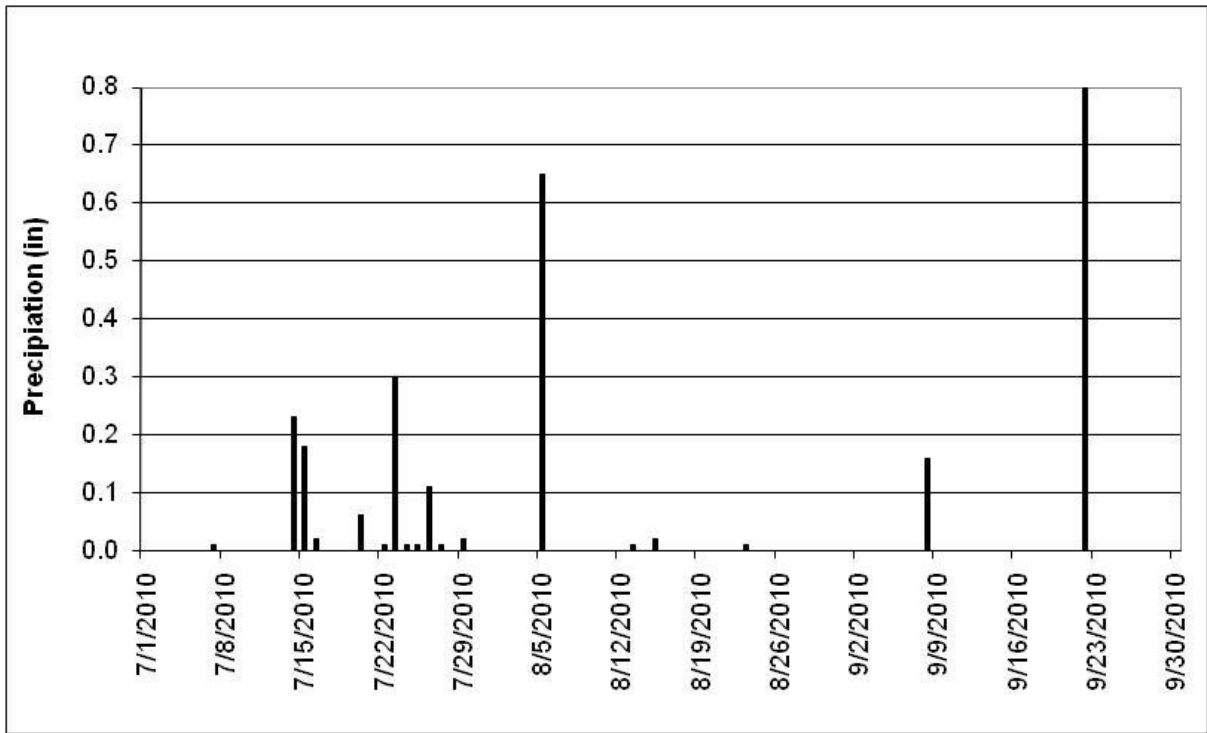
Figure 1. Daily total precipitation (inches), July 2010 – September 2010, from the SMWS.
