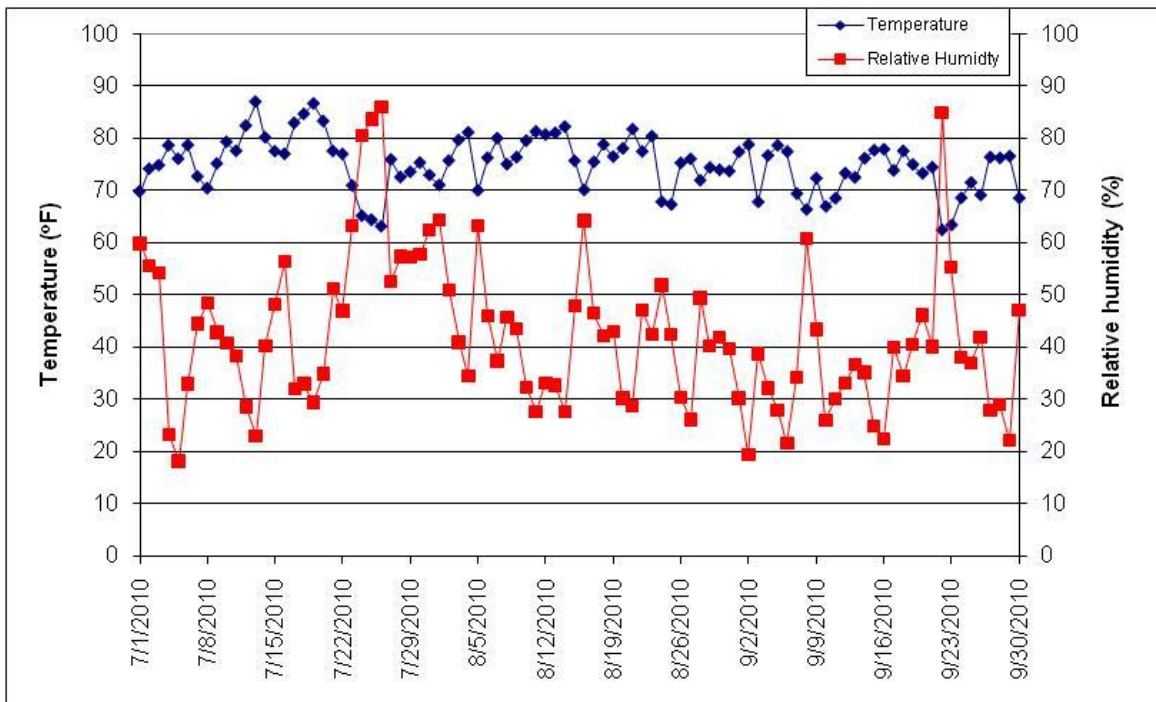
Figure 8. Daily average ambient air temperature and relative humidity, July 1-September 30, 2010.
